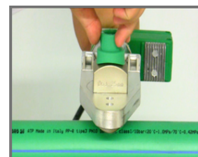
saddle welding
