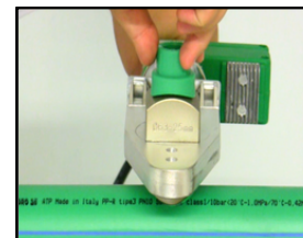
saddle welding
